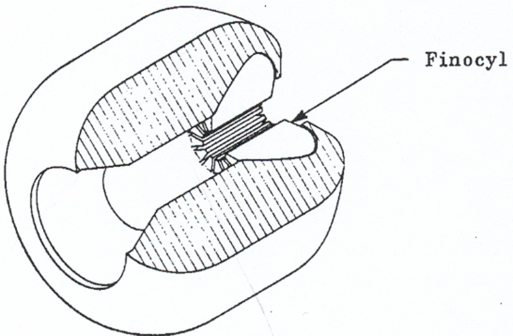
Finocyl configuration
